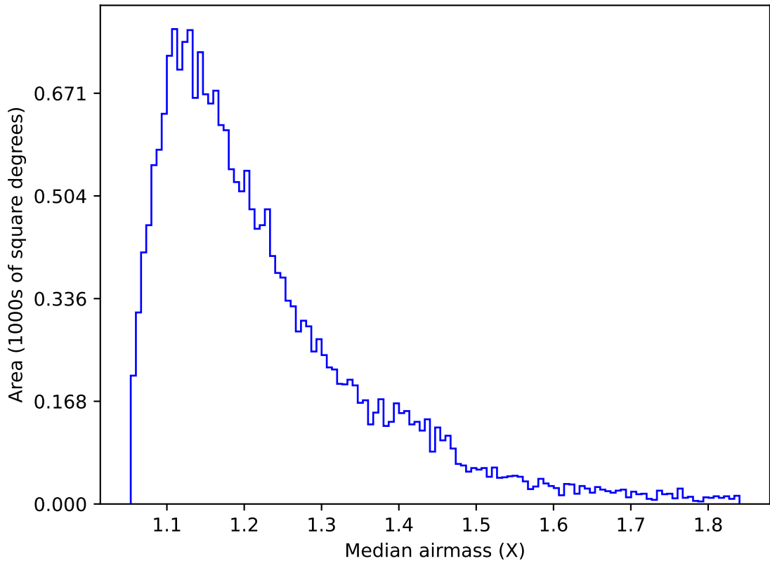
too_elab_r32_d2_ugrizy_v3.4_10yrs Yr 1 u band: Median airmass
