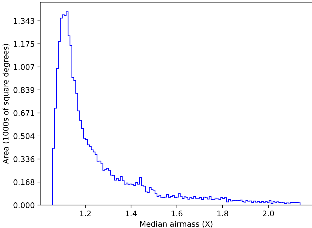
too_elab_r32_d2_ugrizy_v3.4_10yrs Yr 1 r band: Median airmass
