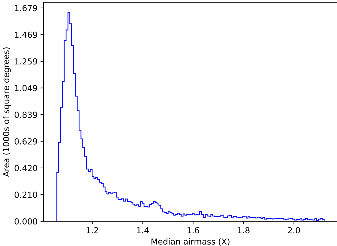
too_elab_r32_d2_ugrizy_v3.4_10yrs Yr 1 i band: Median airmass
