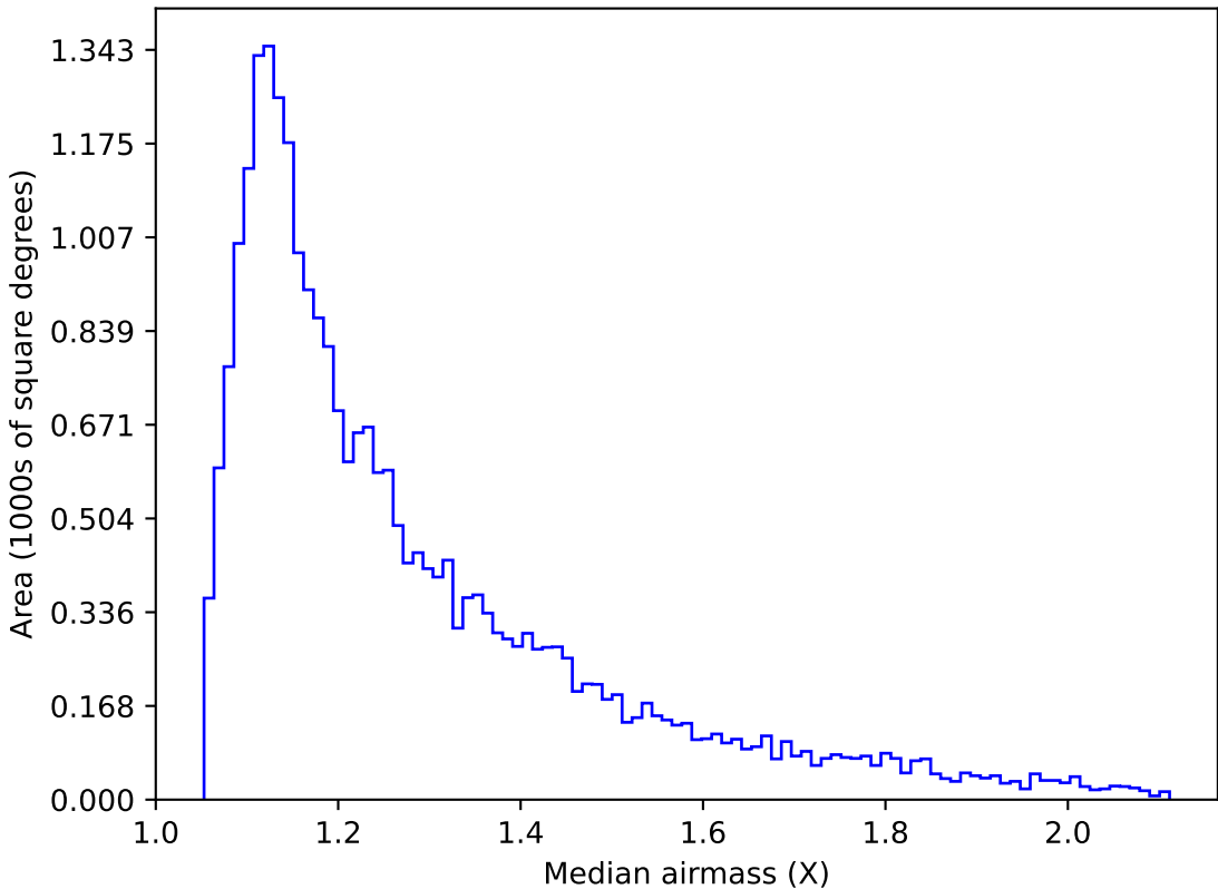
too_elab_r32_d2_ugrizy_v3.4_10yrs Yr 1 g band: Median airmass
