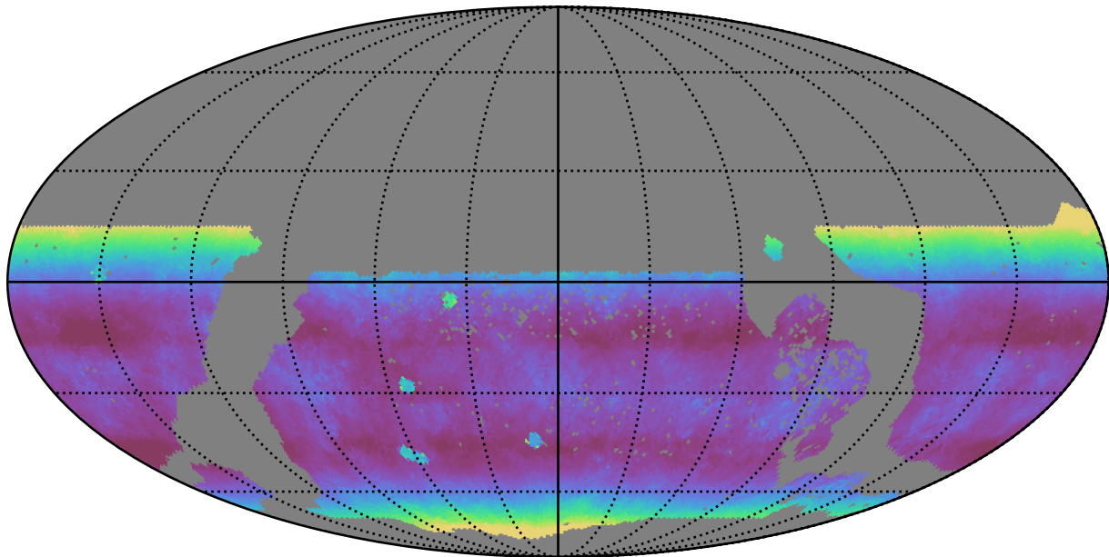
too_elab_r32_d2_ugrizy_v3.4_10yrs WFD z band: Median airmass
