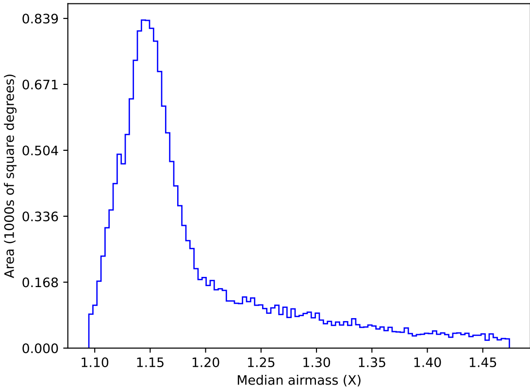
too_elab_r32_d2_ugrizy_v3.4_10yrs WFD y band: Median airmass
