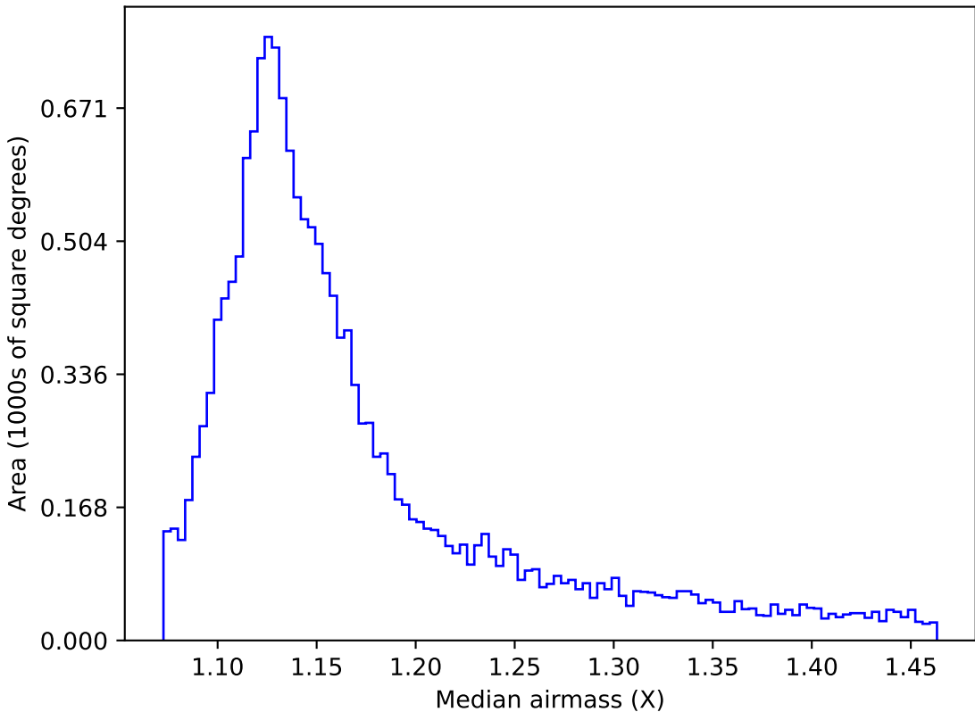
too_elab_r32_d2_ugrizy_v3.4_10yrs WFD r band: Median airmass
