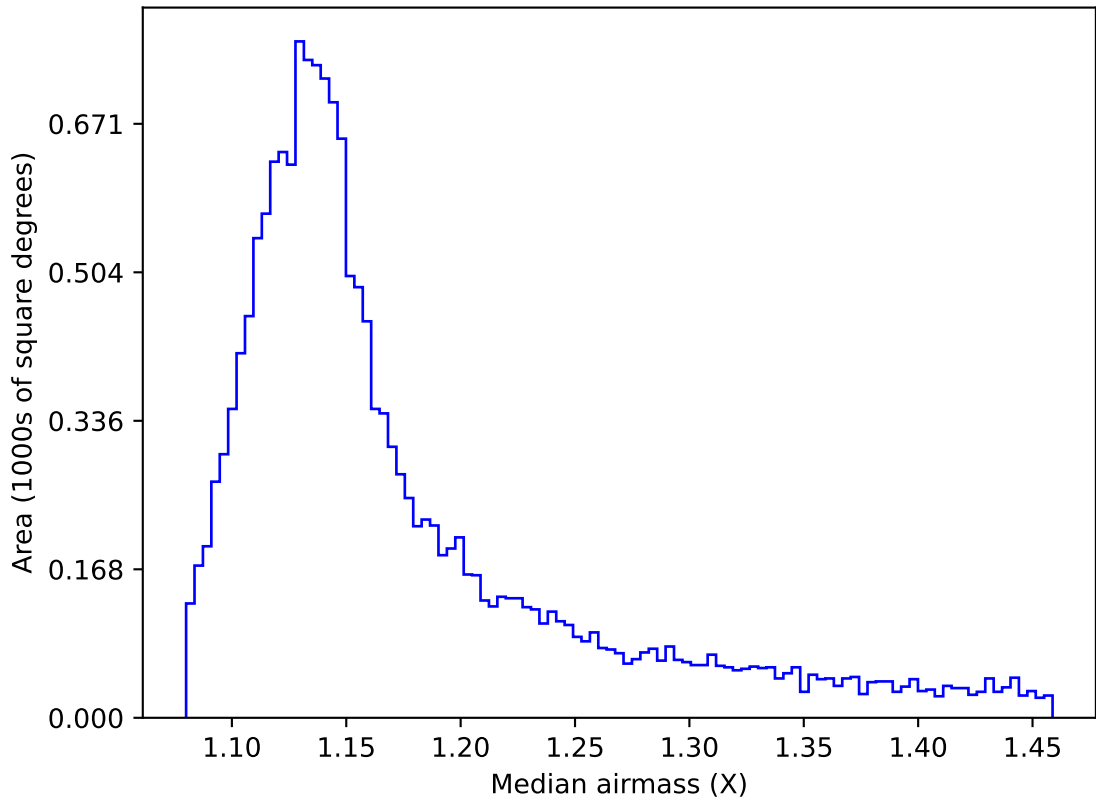
too_elab_r32_d2_ugrizy_v3.4_10yrs WFD i band: Median airmass
