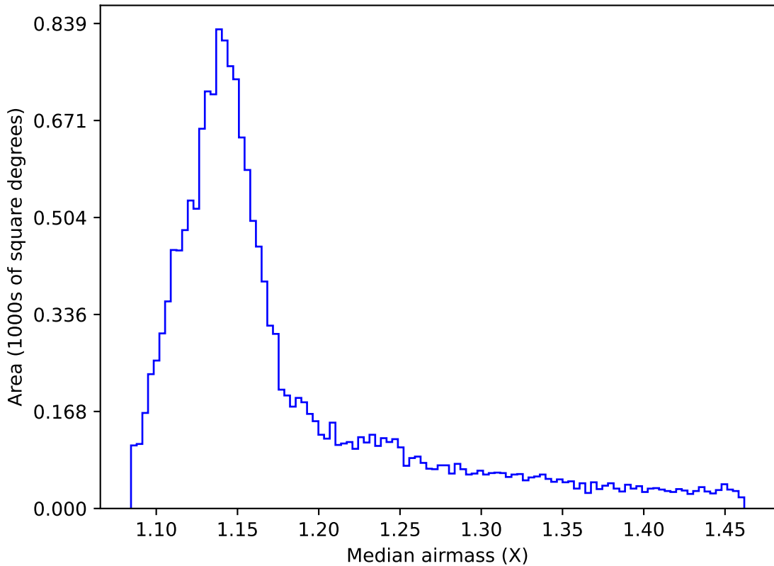
too_elab_r32_d2_ugrizy_v3.4_10yrs WFD all bands: Median airmass
