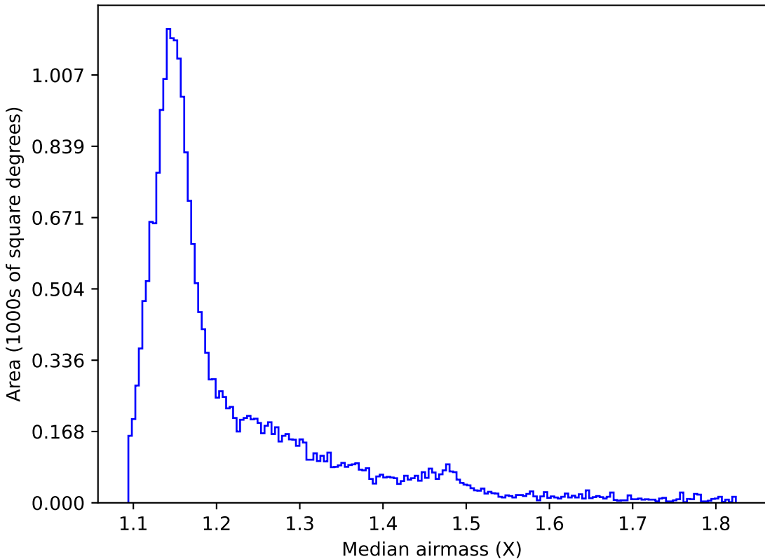
too_elab_r32_d2_ugrizy_v3.4_10yrs All sky y band: Median airmass
