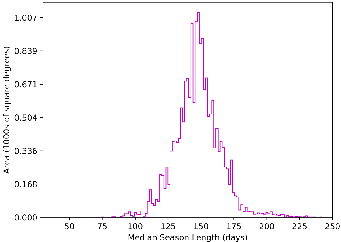
too_elab_r32_d2_ugrizy_v3.4_10yrs WFD z band: Median Season Length
