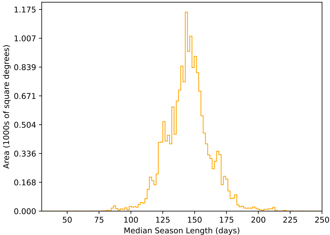
too_elab_r32_d2_ugrizy_v3.4_10yrs WFD r band: Median Season Length
