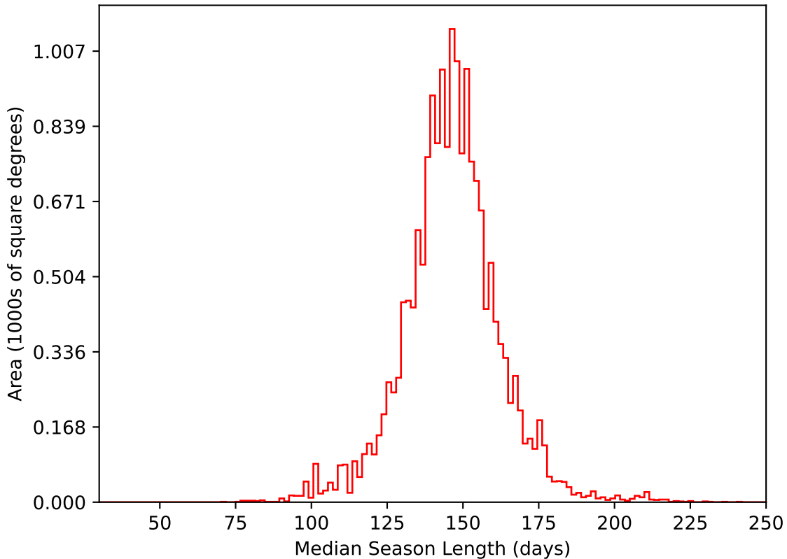
too_elab_r32_d2_ugrizy_v3.4_10yrs WFD i band: Median Season Length
