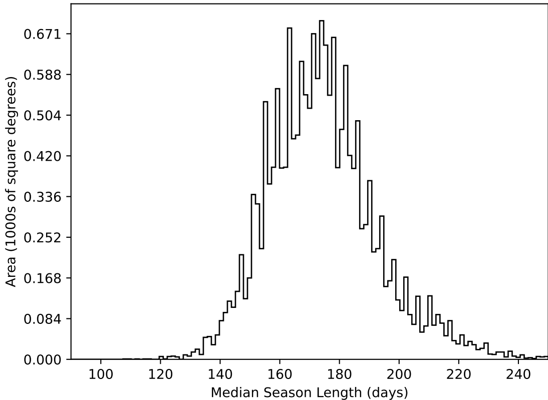
too_elab_r32_d2_ugrizy_v3.4_10yrs WFD all bands: Median Season Length
