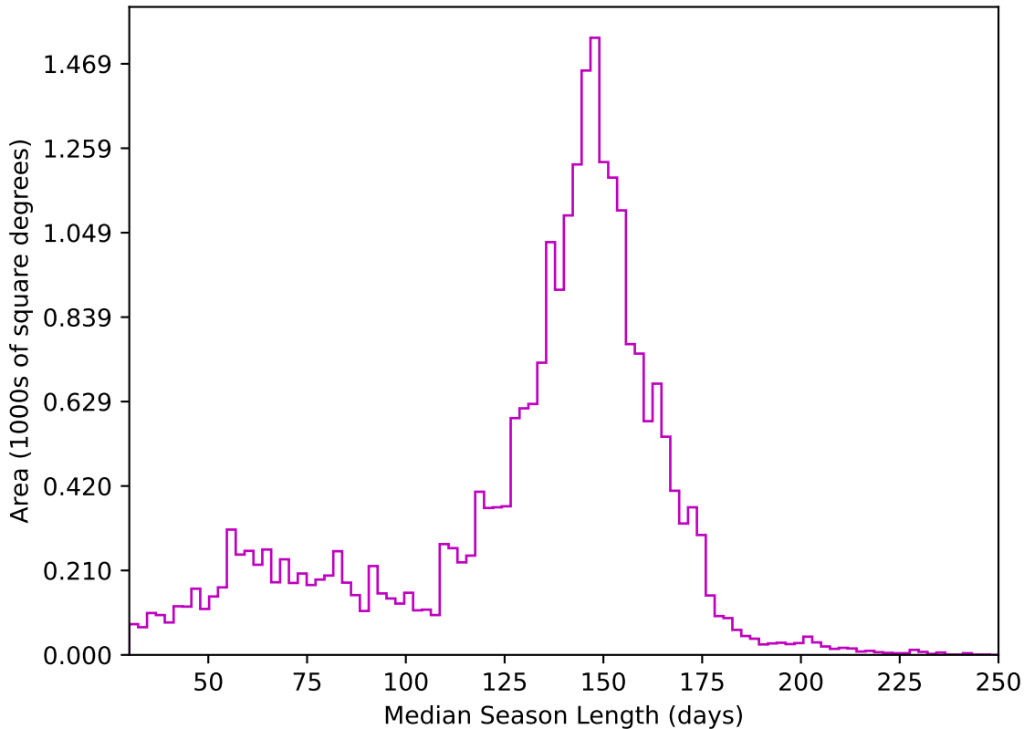
too_elab_r32_d2_ugrizy_v3.4_10yrs All sky z band: Median Season Length
