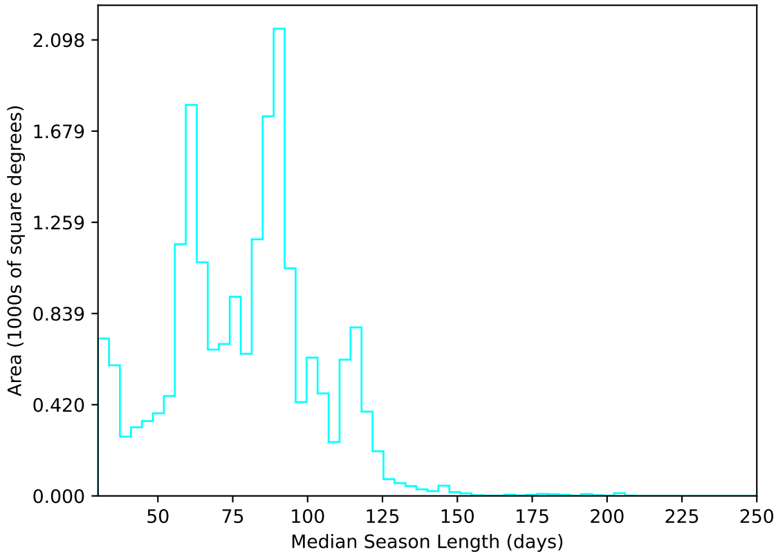
too_elab_r32_d2_ugrizy_v3.4_10yrs All sky u band: Median Season Length
