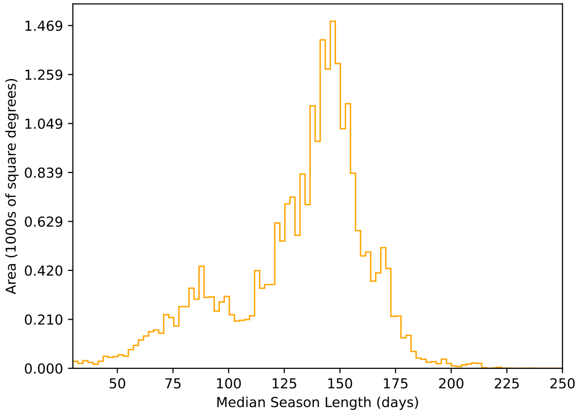
too_elab_r32_d2_ugrizy_v3.4_10yrs All sky r band: Median Season Length
