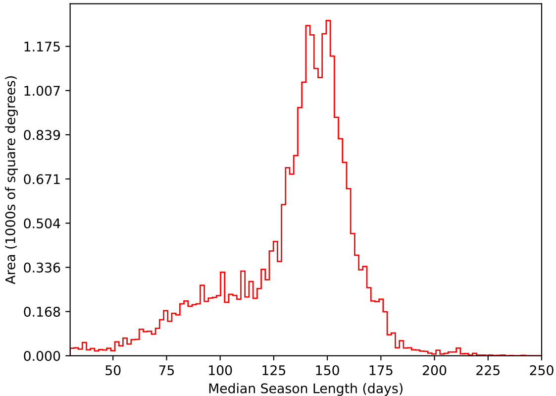
too_elab_r32_d2_ugrizy_v3.4_10yrs All sky i band: Median Season Length
