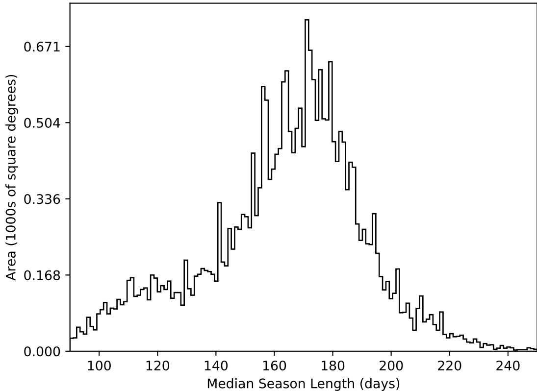
too_elab_r32_d2_ugrizy_v3.4_10yrs All sky all bands: Median Season Length
