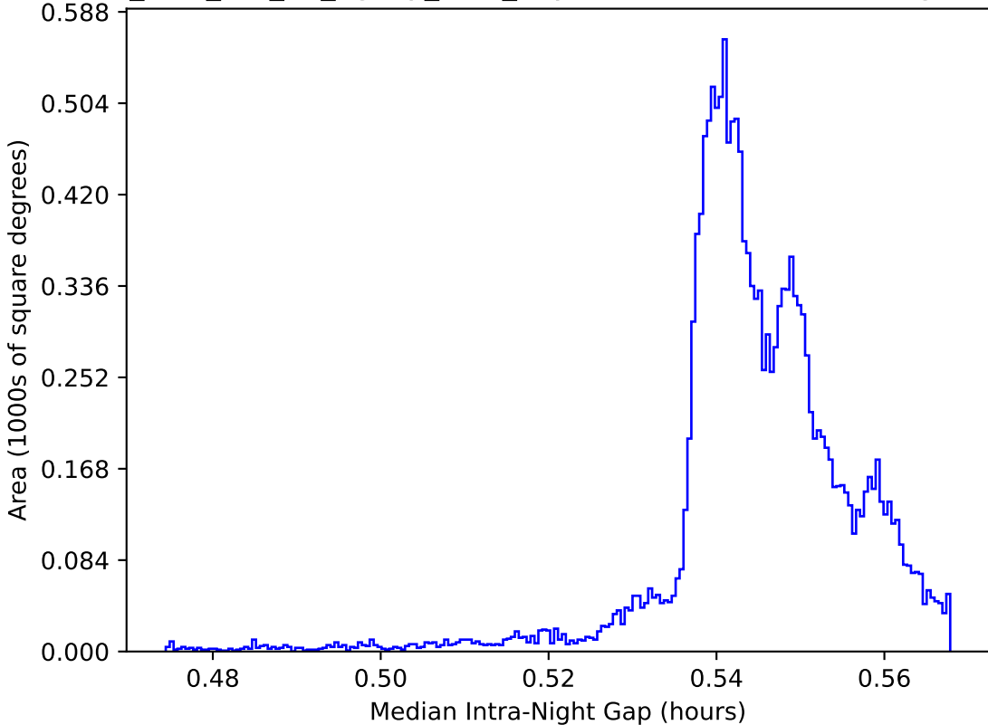
too_elab_r32_d2_ugrizy_v3.4_10yrs WFD: Median Intra-Night Gap
