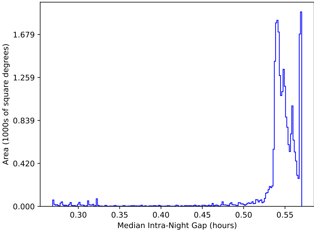
too_elab_r32_d2_ugrizy_v3.4_10yrs All sky: Median Intra-Night Gap
