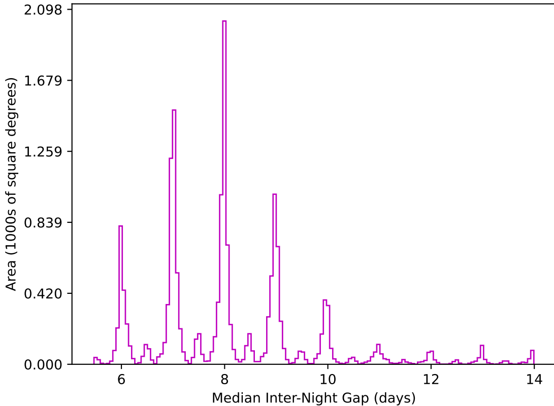
too_elab_r32_d2_ugrizy_v3.4_10yrs WFD z band: Median Inter-Night Gap
