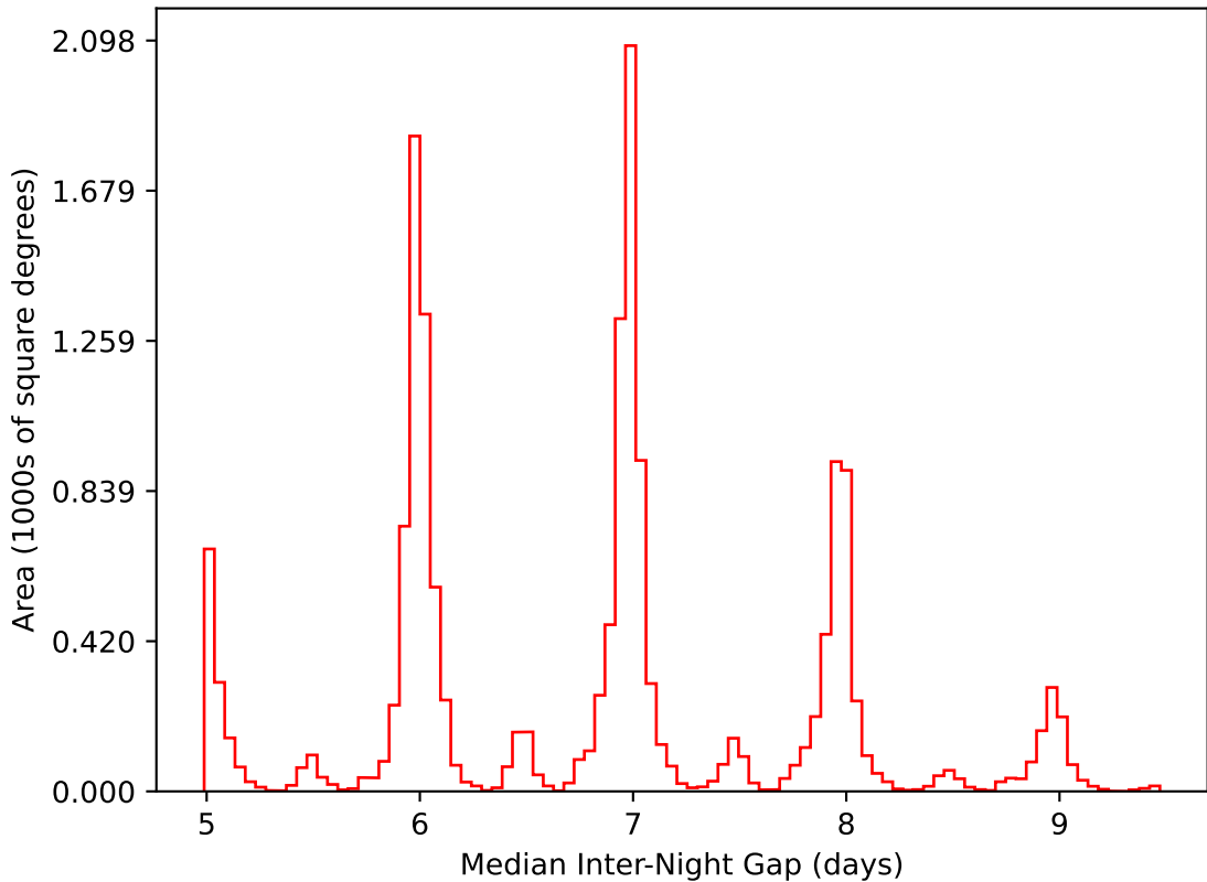
too_elab_r32_d2_ugrizy_v3.4_10yrs WFD i band: Median Inter-Night Gap
