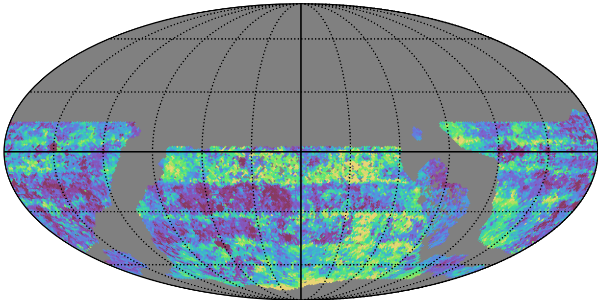
too_elab_r32_d2_ugrizy_v3.4_10yrs WFD g band: Median Inter-Night Gap
