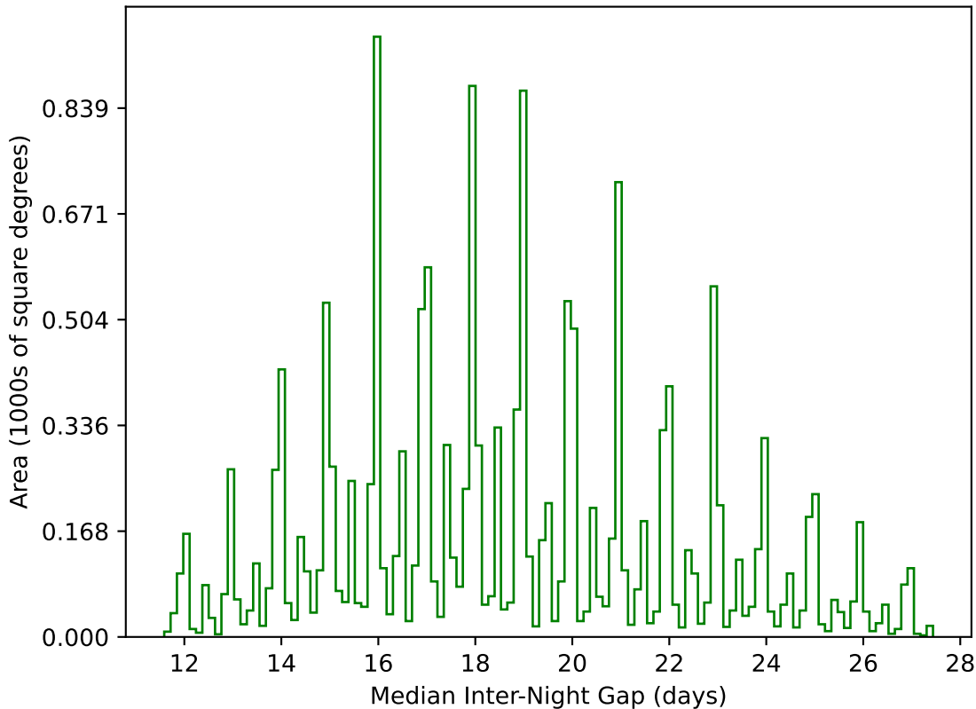
too_elab_r32_d2_ugrizyv3.4_10yrs WFD g band: Median Inter-Night Gap
