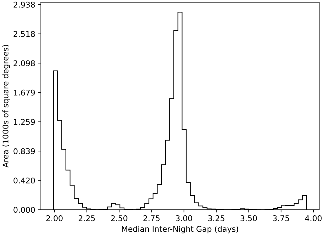
too_elab_r32_d2_ugrizy_v3.4_10yrs WFD all bands: Median Inter-Night Gap
