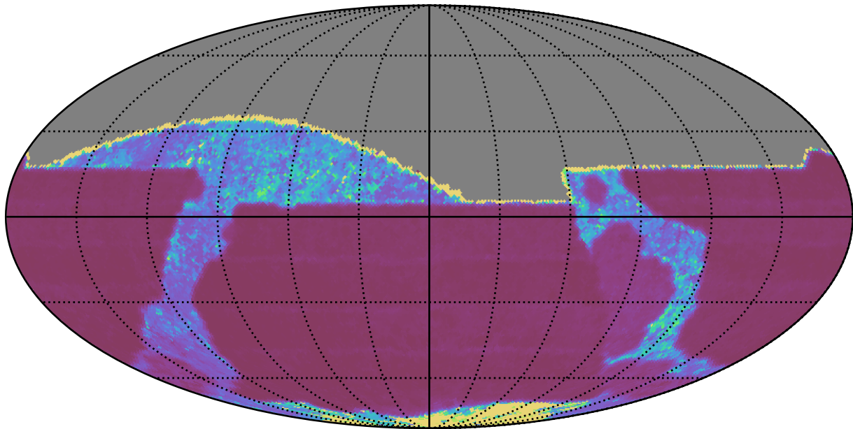
too_elab_r32_d2_ugrizy_v3.4_10yrs All sky z band: Median Inter-Night Gap
