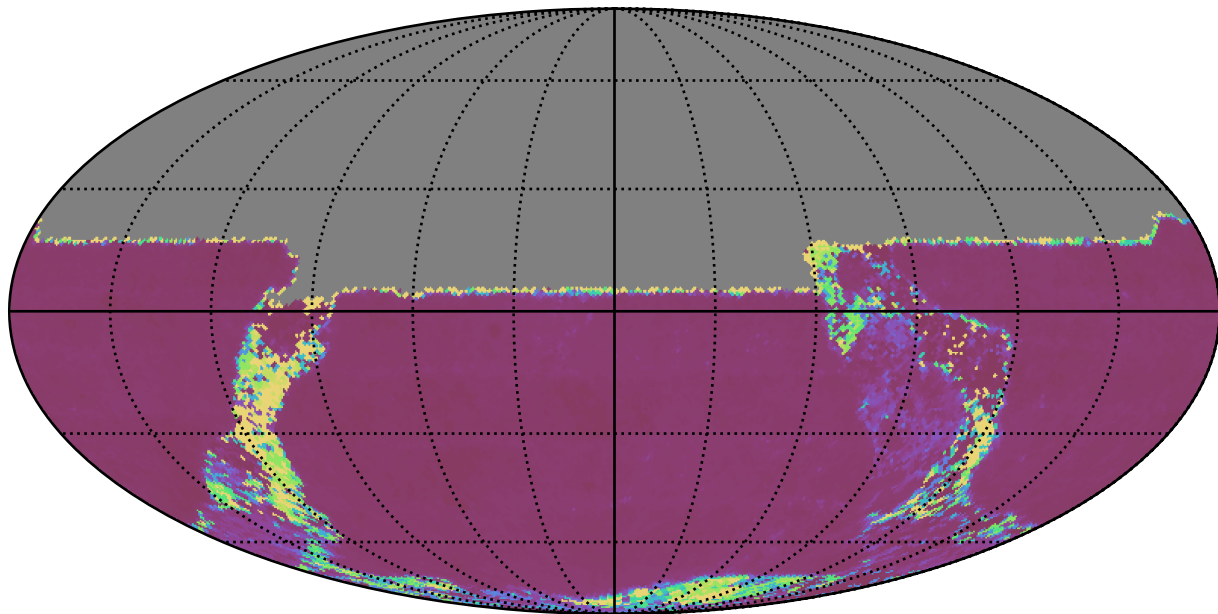
too_elab_r32_d2_ugrizy_v3.4_10yrs All sky u band: Median Inter-Night Gap
