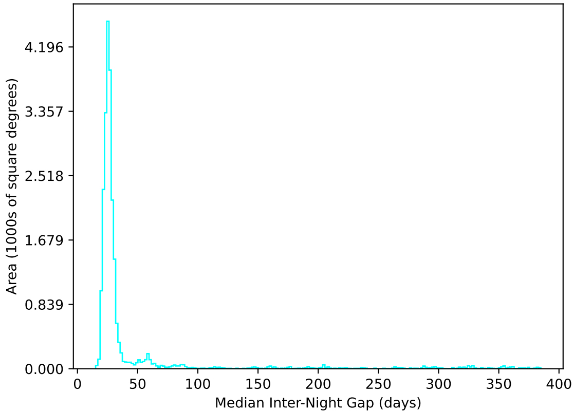
too_elab_r32_d2_ugrizy_v3.4_10yrs All sky u band: Median Inter-Night Gap
