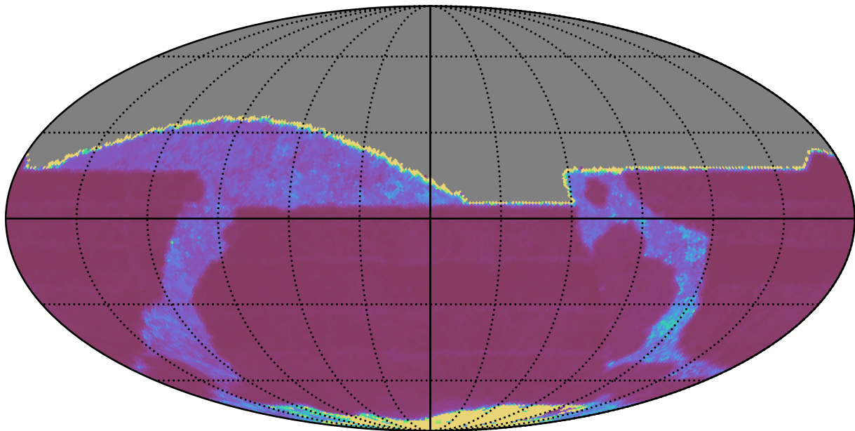
too_elab_r32_d2_ugrizy_v3.4_10yrs All sky r band: Median Inter-Night Gap
