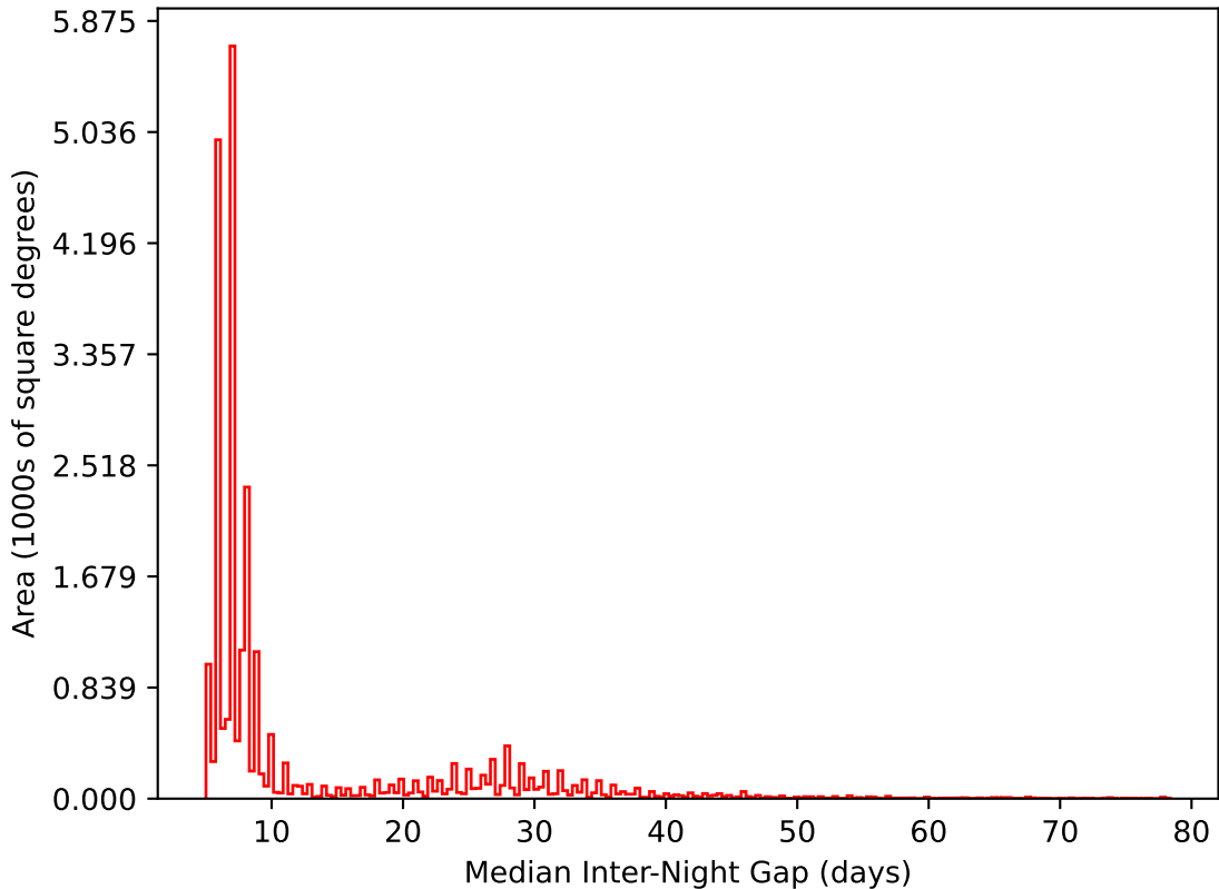
too_elab_r32_d2_ugrizy_v3.4_10yrs All sky i band: Median Inter-Night Gap
