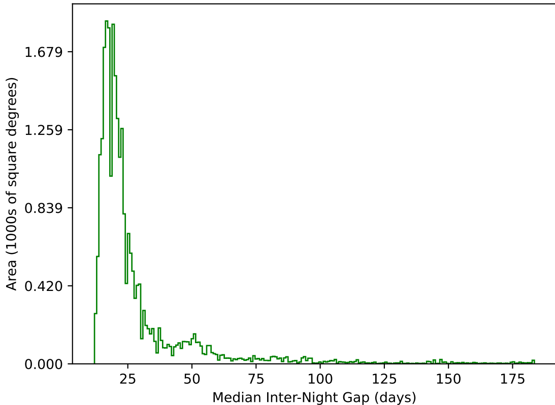
too_elab_r32_d2_ugrizy_v3.4_10yrs All sky g band: Median Inter-Night Gap
