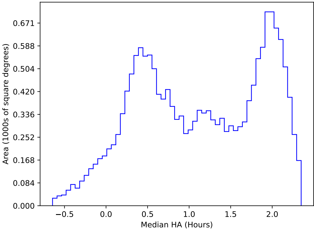
too_elab_r32_d2_ugrizy_v3.4_10yrs WFD z band: Median HA
