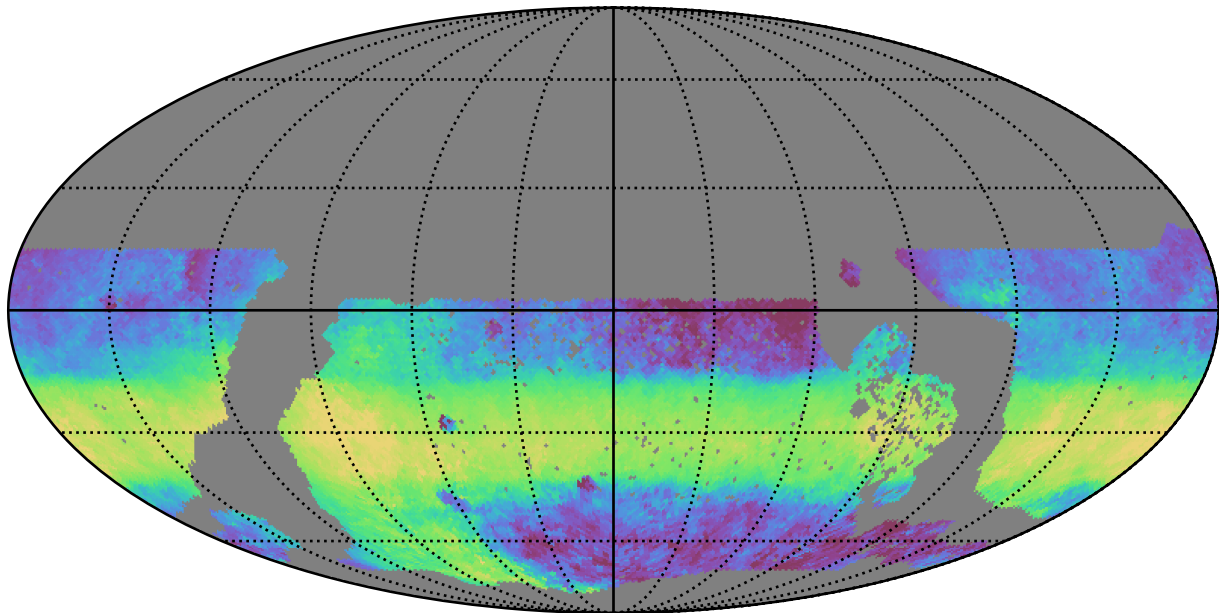
too_elab_r32_d2_ugrizy_v3.4_10yrs WFD y band: Median HA
