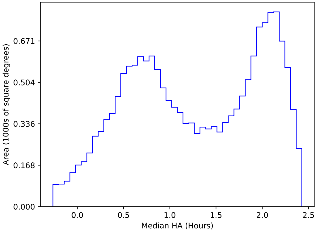
too_elab_r32_d2_ugrizy_v3.4_10yrs WFD y band: Median HA
