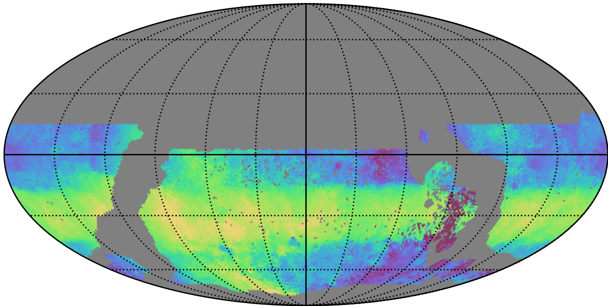
too_elab_r32_d2_ugrizy_v3.4_10yrs WFD u band: Median HA
