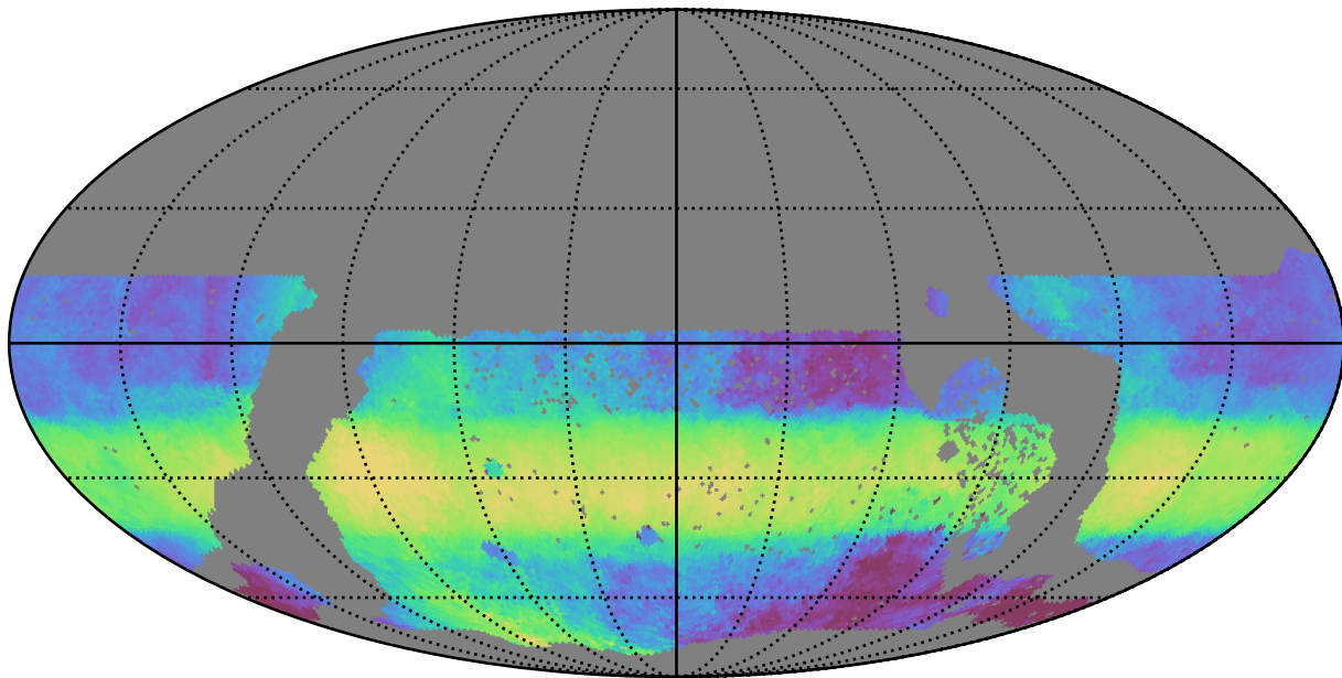
too_elab_r32_d2_ugrizy_v3.4_10yrs WFD r band: Median HA
