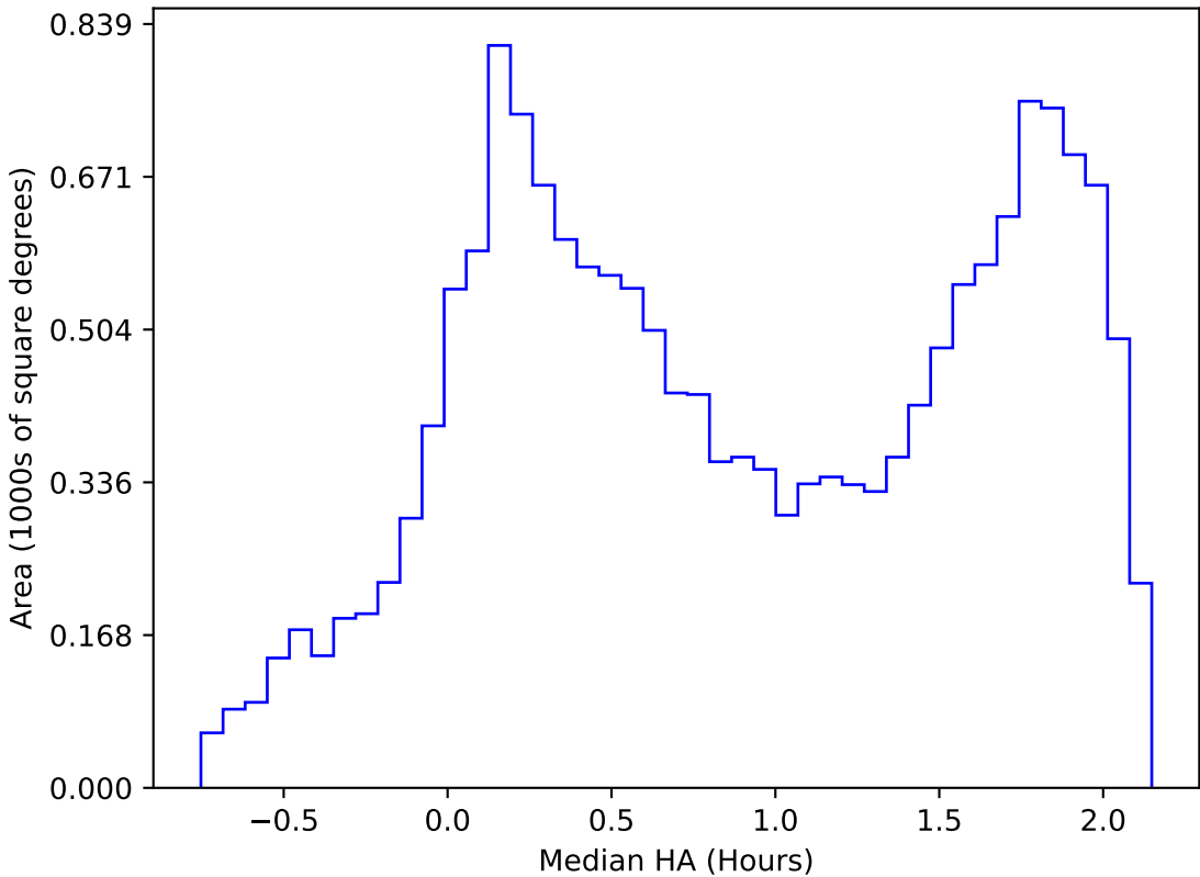
too_elab_r32_d2_ugrizy_v3.4_10yrs WFD r band: Median HA
