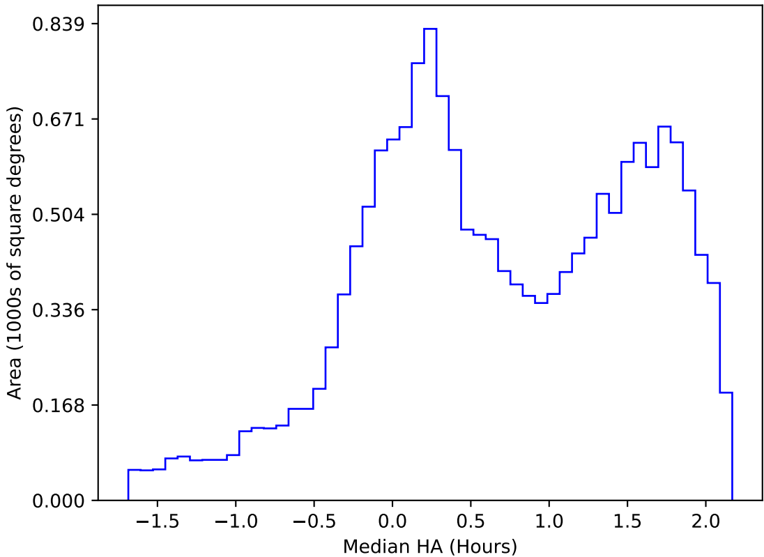
too_elab_r32_d2_ugrizy_v3.4_10yrs WFD g band: Median HA
