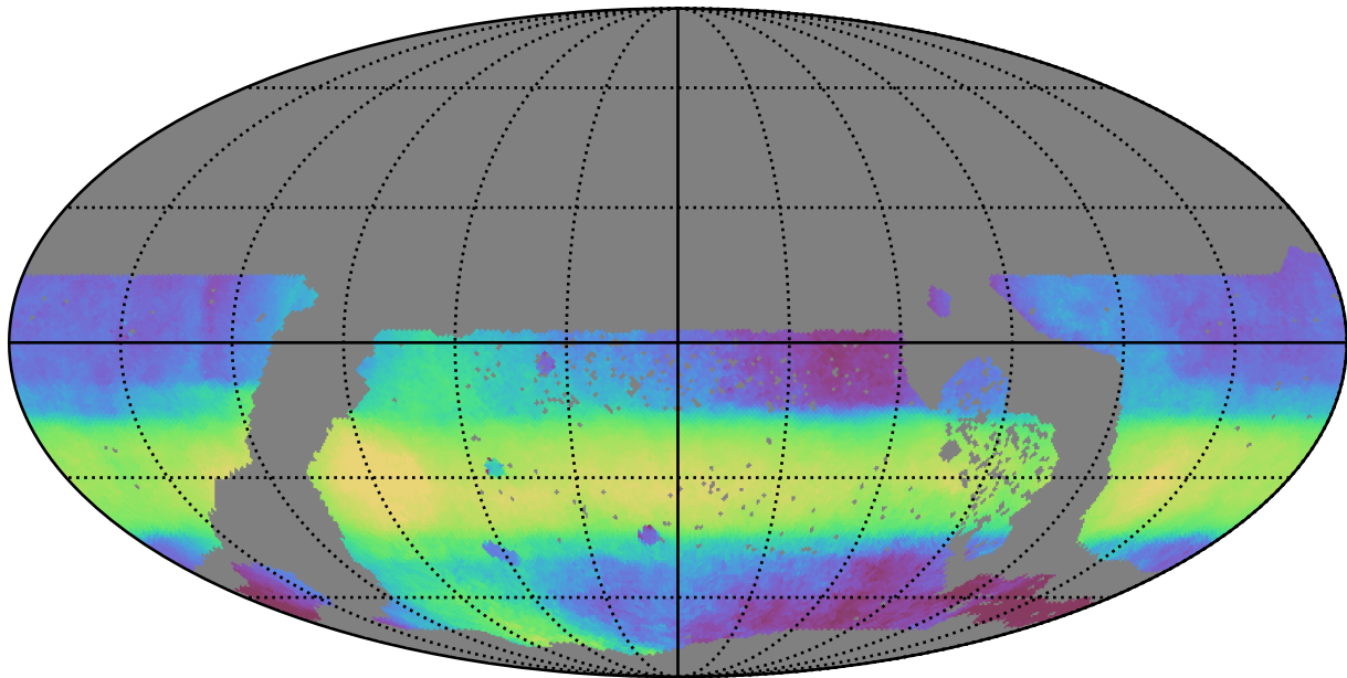
too_elab_r32_d2_ugrizy_v3.4_10yrs WFD all bands: Median HA
