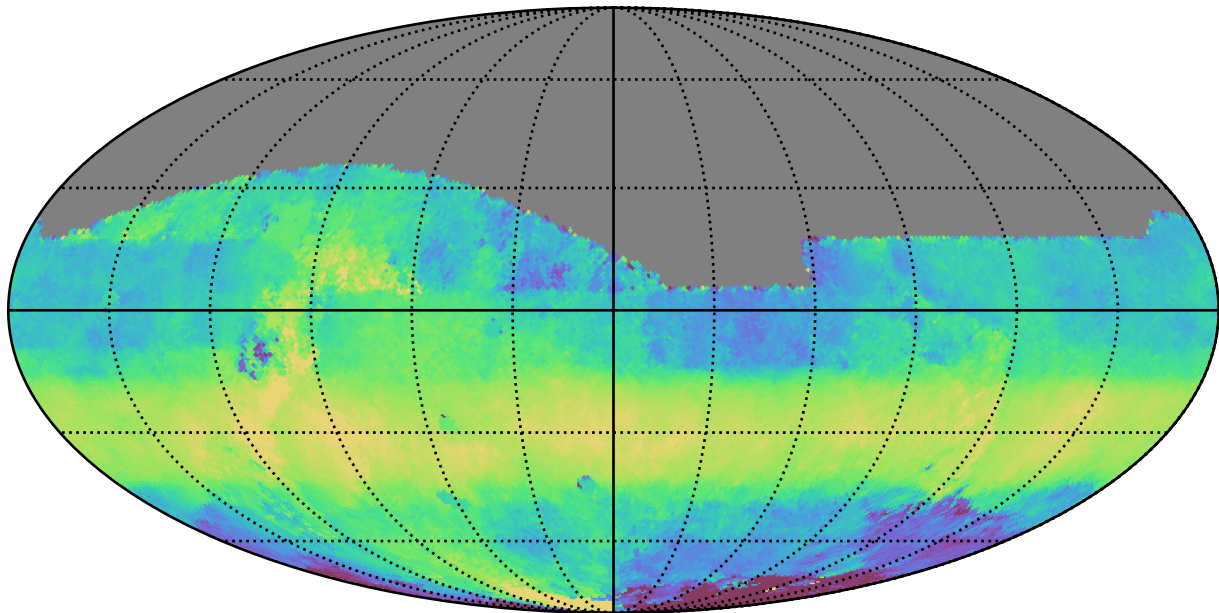
too_elab_r32_d2_ugrizy_v3.4_10yrs All sky z band: Median HA
