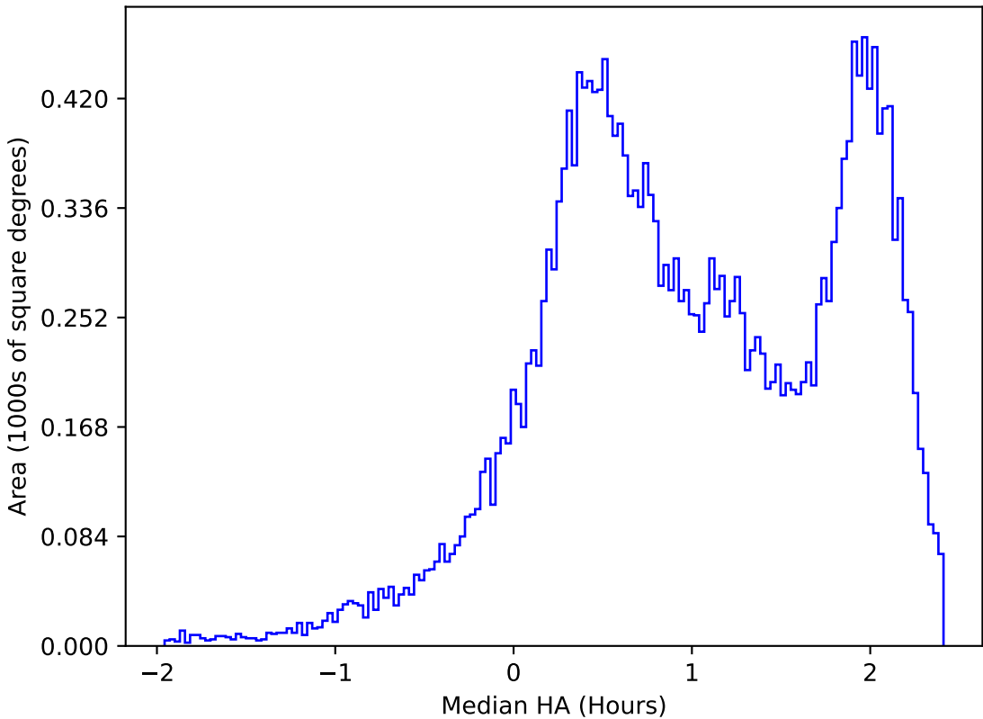
too_elab_r32_d2_ugrizy_v3.4_10yrs All sky z band: Median HA
