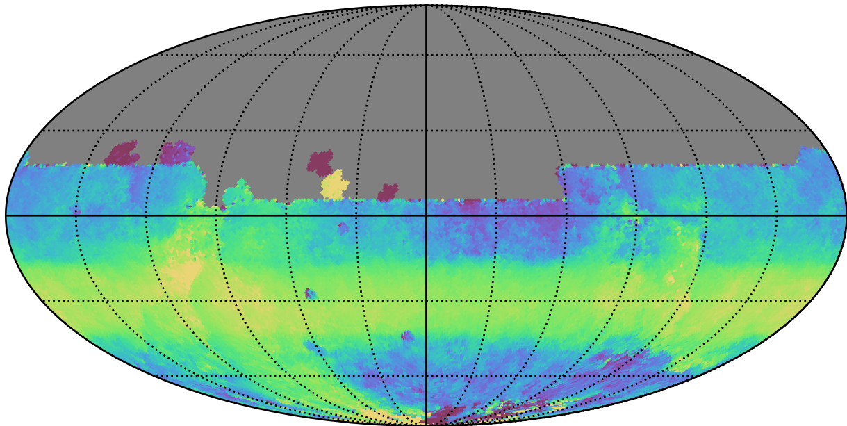
too_elab_r32_d2_ugrizy_v3.4_10yrs All sky y band: Median HA
