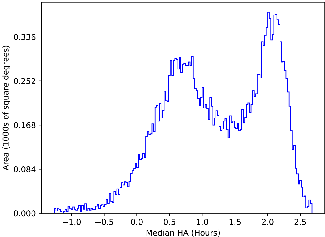
too_elab_r32_d2_ugrizy_v3.4_10yrs All sky y band: Median HA
