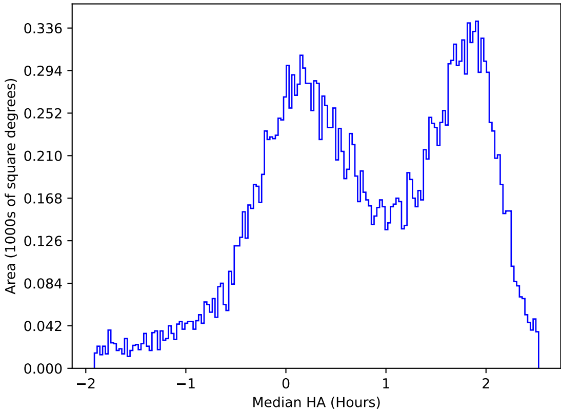
too_elab_r32_d2_ugrizy_v3.4_10yrs All sky u band: Median HA
