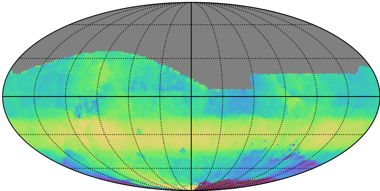
too_elab_r32_d2_ugrizy_v3.4_10yrs All sky r band: Median HA
