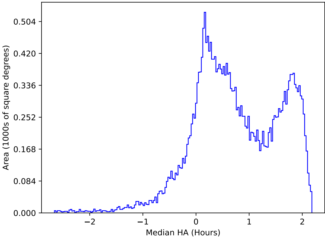
too_elab_r32_d2_ugrizy_v3.4_10yrs All sky r band: Median HA
