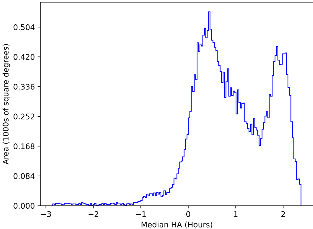
too_elab_r32_d2_ugrizy_v3.4_10yrs All sky i band: Median HA
