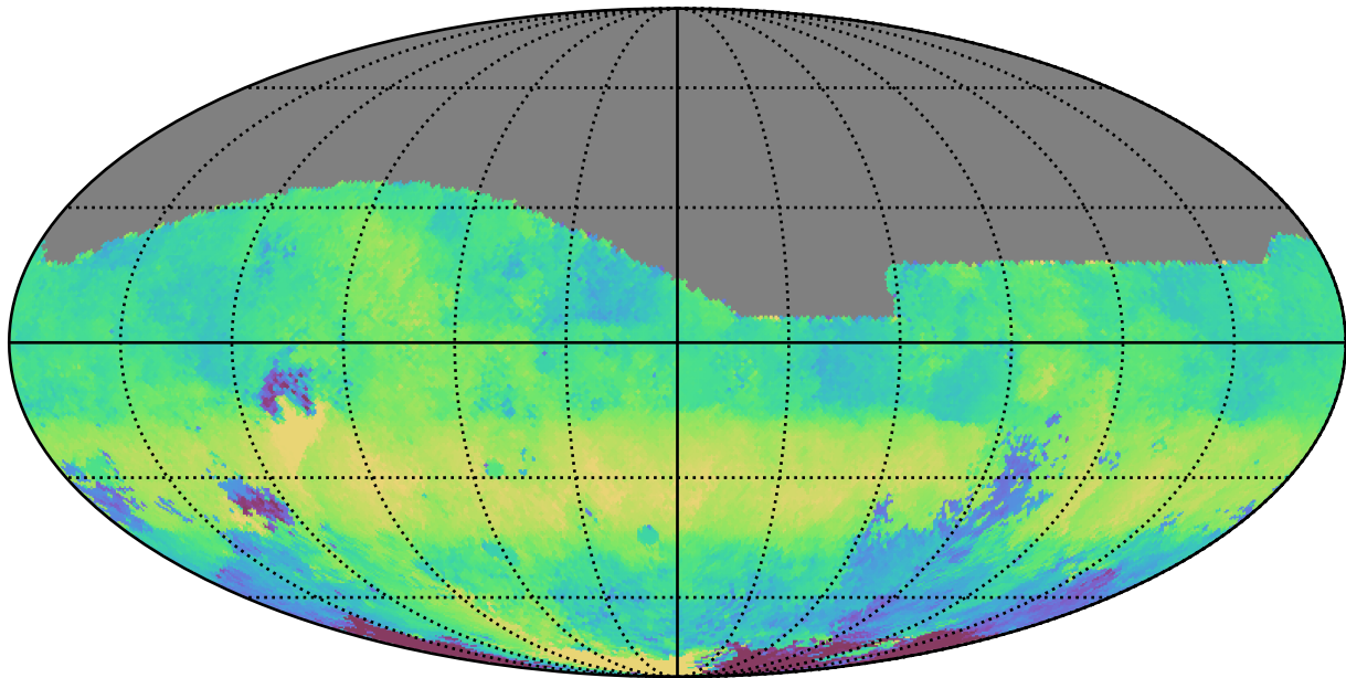
too_elab_r32_d2_ugrizy_v3.4_10yrs All sky g band: Median HA
