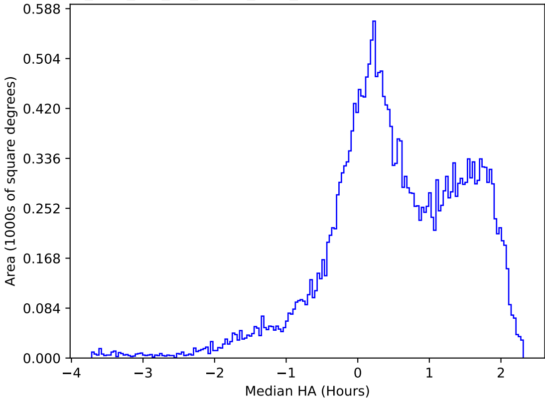
too_elab_r32_d2_ugrizy_v3.4_10yrs All sky g band: Median HA
